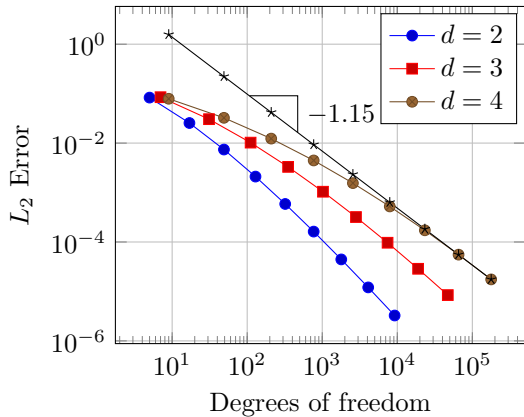
Convergence Plot
